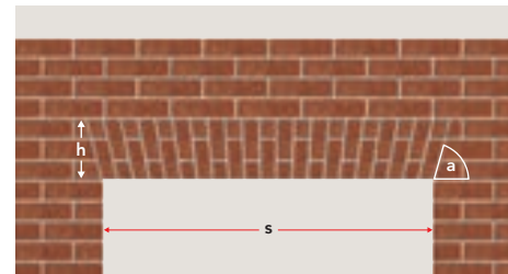
Front elevation notes the essential measurements required to specify the Lightweight Flat Gauge Header.
