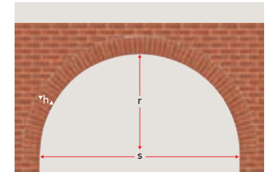
Front elevation notes the essential measurements required to specify the Semi Circular Arch BSFL.
