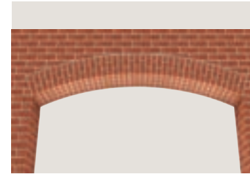
View showing the underside of IG's Segmental Arch BSFL. This illustrates how the brickwork returns under the soffit of the lintel to ensure no steelwork is visible on the outer leaf.
