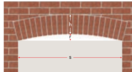
Front elevation notes the essential measurements required to specify the Lightweight Segmental Arch Header.
