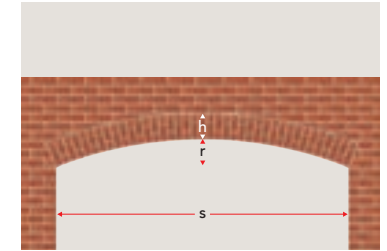
Front elevation notes the essential measurements required to specify the Segmental Arch BSFL.
